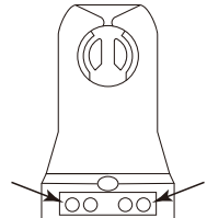
Non-shunted lampholder
