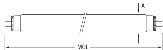
Bi-pin G5 Base
